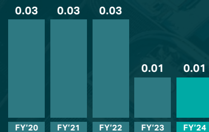
Multiyear LWCR Trend
